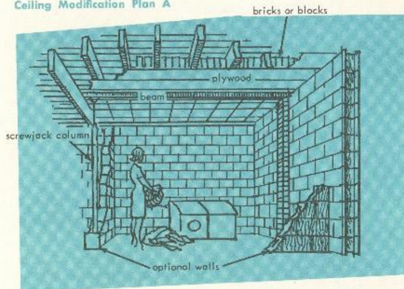
Ceiling Modification Plan A
